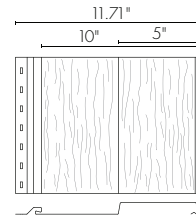
5" X 5" BOARD & BATTEN
