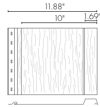
10" BOARD & BATTEN
