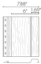
6" BOARD & BATTEN
